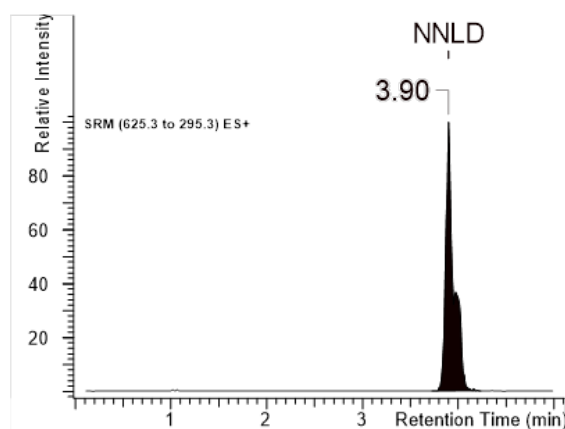
Figure 3. Representative MRM (625m/z to 295m/z) chromatogram for NNLD at LOQ level
