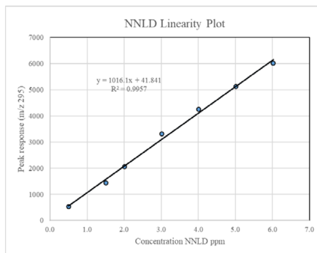
Figure 5. Linearity plot for NNLD
