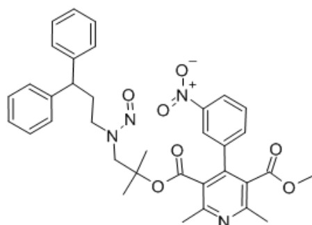
Figure 2. N-nitroso-desmethyl-lercanidipine impurity D(NNLD) chemical structure
