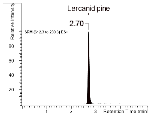
Figure 4. Representative MRM (612m/z to 280m/z) chromatogram for Lercanidipine drug substance
