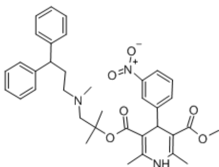
Figure 1. Lercanidipine(LD) chemical structure
