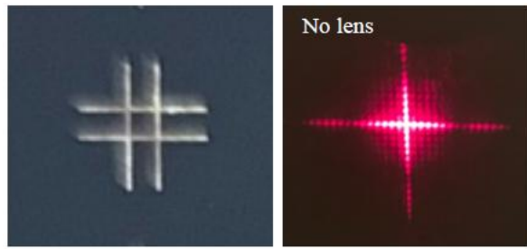
Figure A.1.0. typical orthogonal cross double slit and its pattern
