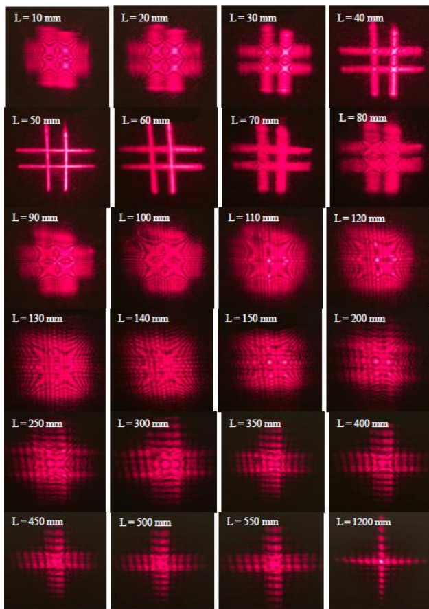
Figure A.1. Evolution of Pre-Particle Pattern to Particle Pattern to Transition Patterns to Interference Patterns
