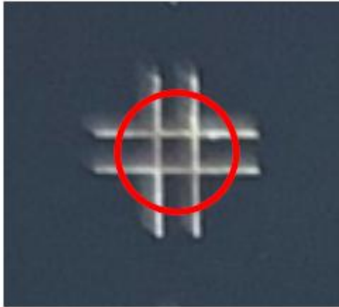
Figure 2.2. Laser beam illuminating cross double slit
