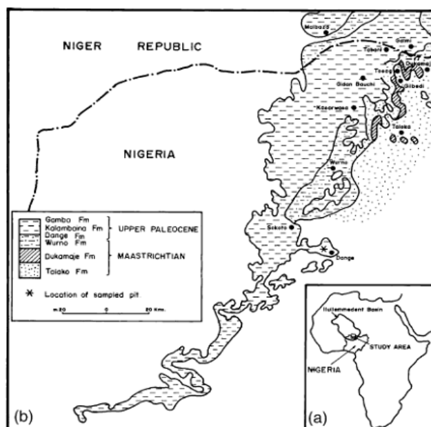
Figure 1. (a) Map of Africa, showing the Sokoto sub-basin, Northwest Nigeria in relation to the Iullemeden basin. Inset: Location of (b). (b) Simplified geological map of the southeastern sector marine and marginal facies of Illemeden basin, Sokoto sub-basin (Okosun, 1997)
