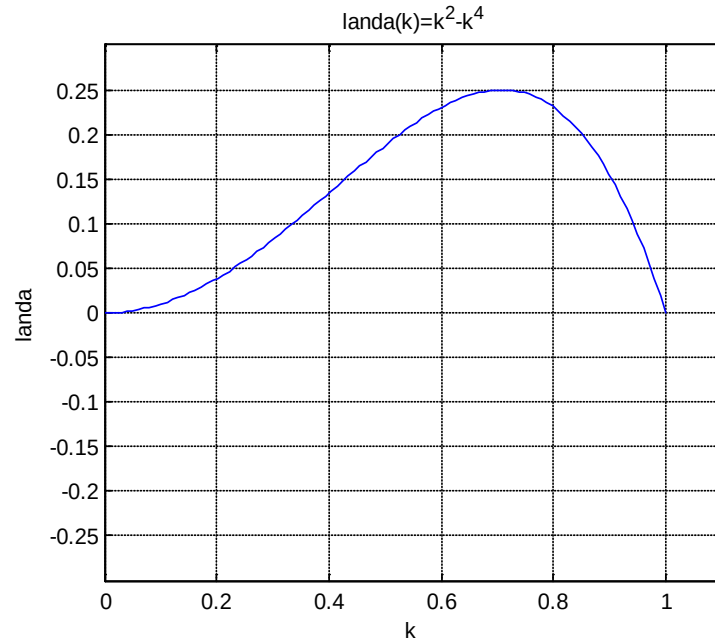
Figure 1. The growth rate \lambda(k) for perturbations of the form e^{\lambda t} e^{ikx} to the zero solution of the Kuramoto-Sivashinsky (K-S) equation
