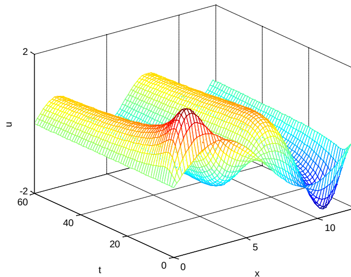
Figure 5. Time evolution of the numerical solution of the Kuramoto-Sivashinsky up to t = 60 with the initial condition u_1(x) = \sin(x/2), x \in [0, 4\pi]
