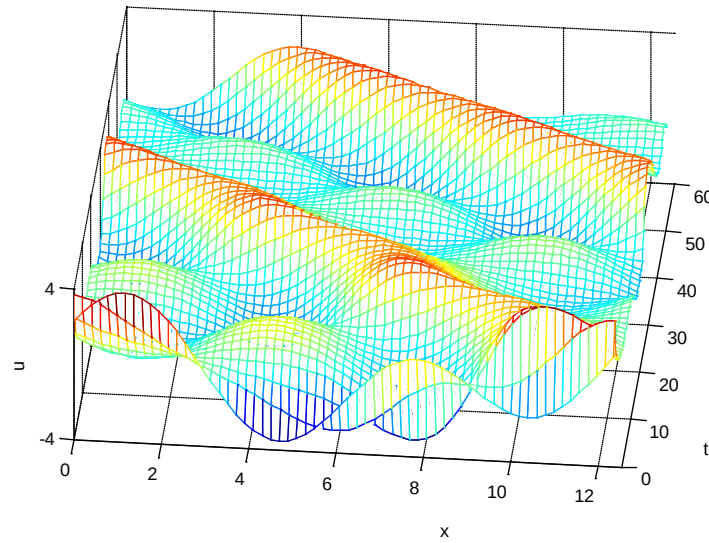
Figure 4. Time evolution of the numerical solution of the Kuramoto-Sivashinsky up to t = 60 with the initial condition
