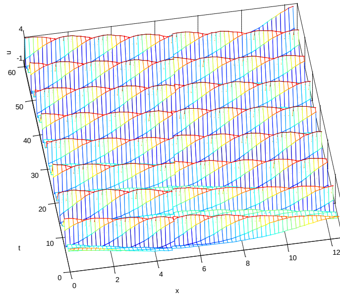
Figure 2. Time evolution of the numerical solution of the Kuramoto-Sivashinsky up to t = 60 with the initial condition u_1(x) = e^{\cos\left(\frac{x}{2}\right)}, x \in [0, 4\pi]
