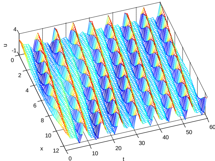
Figure 3. Time evolution of the numerical solution of the Kuramoto-Sivashinsky up to t = 60 with the initial condition u_1(x) = e^{\cos\left(\frac{x}{2}\right)}, x \in [0, 4\pi]
