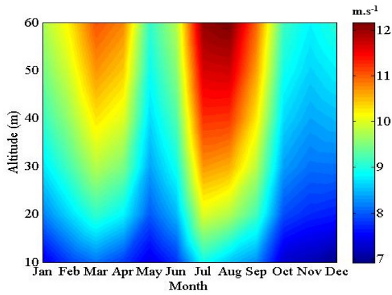
Figure 10. Variation of the wind speed giving the maximum energy as a function of the altitude (2011-2014)
