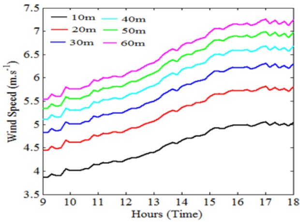
Figure 5. Annual distribution of wind speed during the convective diurnal cycle (2011-2014)
