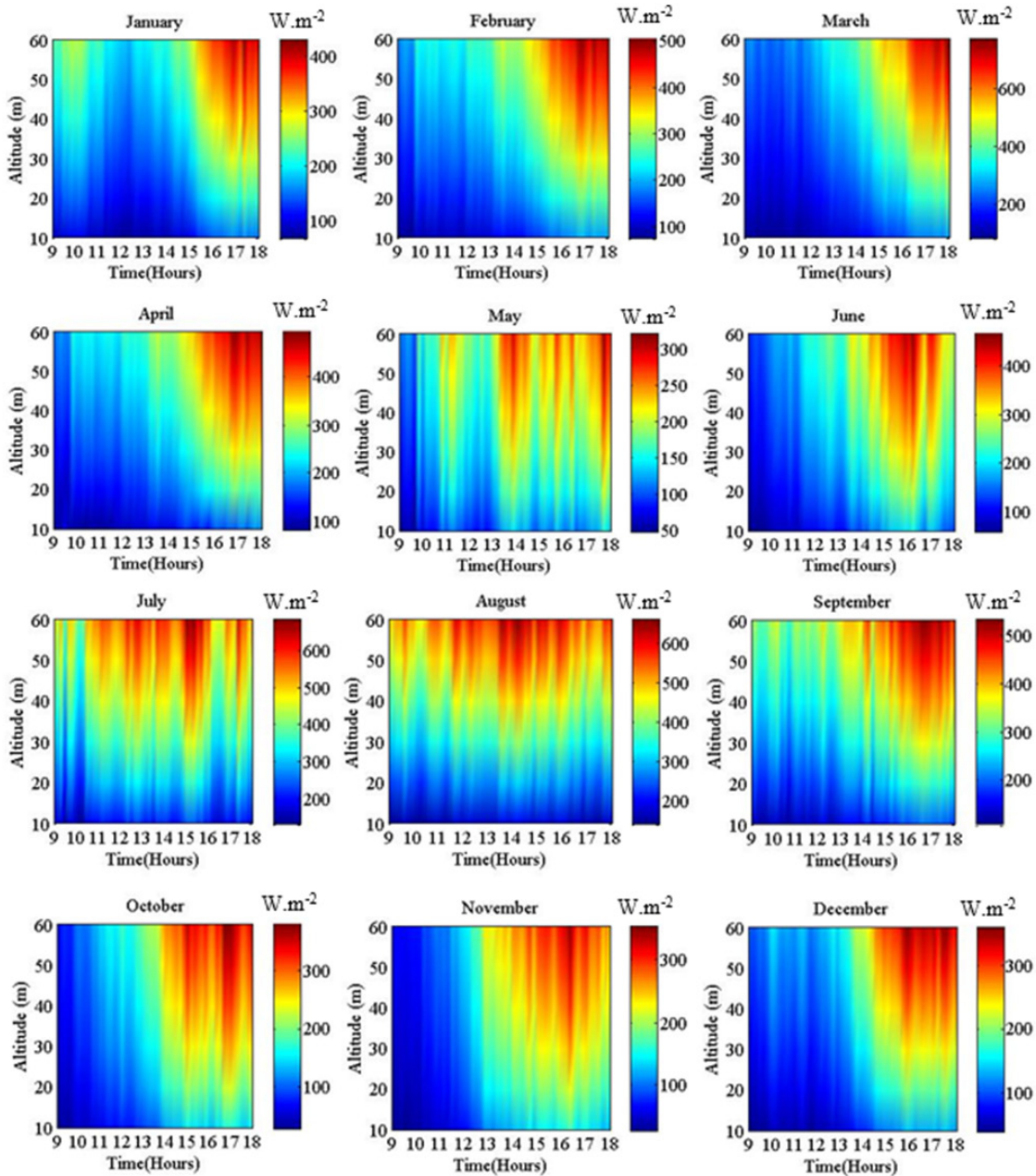
Figure 11. Daily monthly variation of wind energy density from 10 to 60 m at Cotonou Benin (2011-2014)
