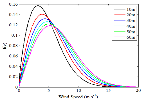
Figure 9. Annual frequency distribution of wind speeds from Weibull model (2011-2014)
