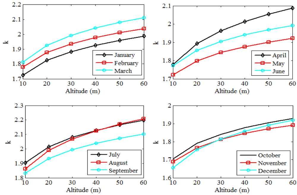
Figure 6. Variation of shape parameter k as a function of altitude (2011-2014)
