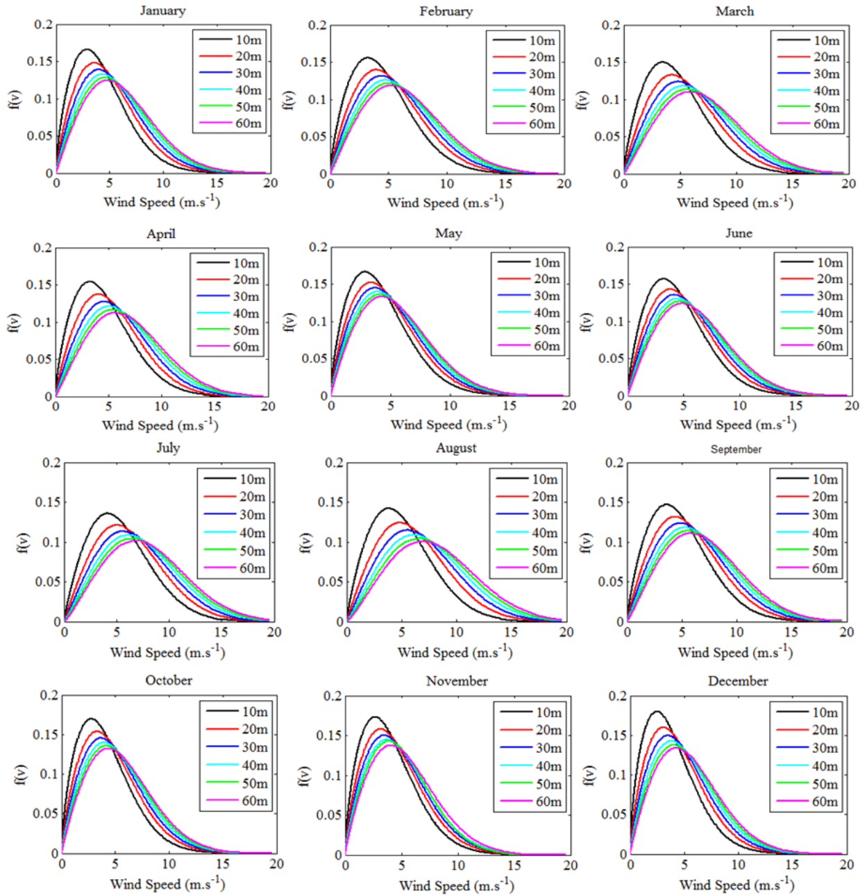
Figure 8. Monthly frequency distribution of wind speeds from Weibull model (2011-2014)
