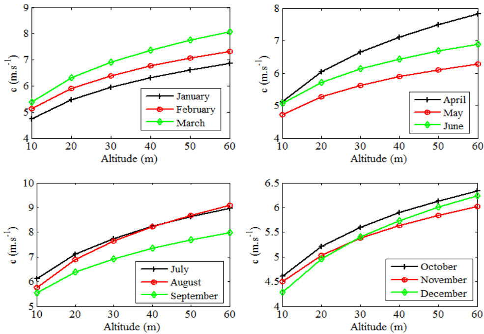
Figure 7. Variation of the scale parameter c as a function of altitude (2011-2014)
